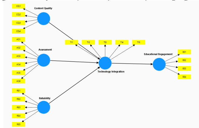
Fig. 2. Measurement Model
