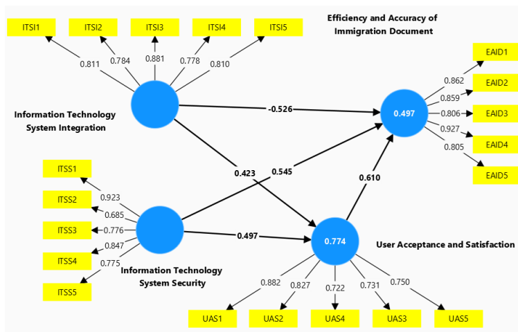
Fig. 2. Validity Testing
