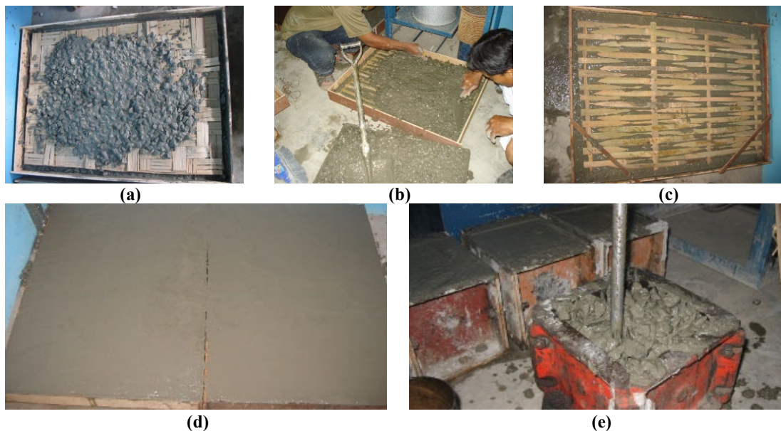
Fig. 2. Test concrete specimen preparation process. (a) Gedhek-type woven bamboo blade test object (D1), (b) bamboo blade type test object (D2), (c) Sasak-type woven bamboo blade test object (D3), (d) finished molding test object, (e) and manufactured concrete cube.
