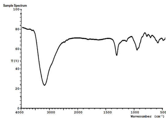
Fig. 1. FTIR of ternary oxide nanoparticles of iron, silver, and vanadium from extracts of Psidium guajava Extract.
