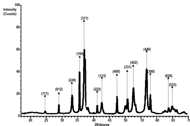
Fig. 4. the XRD pattern of Psidium guajava Extract-Derived Ternary Oxides of Iron, Vanadium, and Silver Nanoparticles synthesized using Psidium guajava plant extract.
