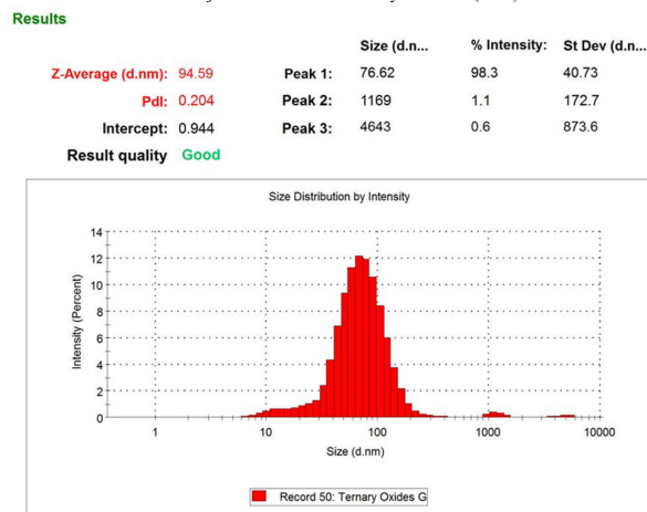
Fig. 2. Dynamic Light Scattering Analysis of Psidium guajava Extract-Derived Ternary Oxides of Iron, Vanadium, and Silver Nanoparticles
