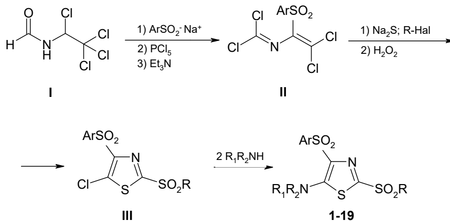
Scheme 1. Synthesis of 2,4-disulfonylsubstituted 5-aminothiazoles 1-19
