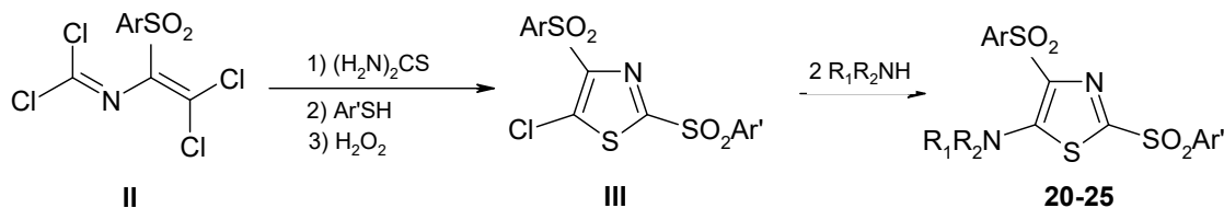
Scheme 2. Synthesis of 2,4-disulfonylsubstituted 5-aminothiazoles 20-25
