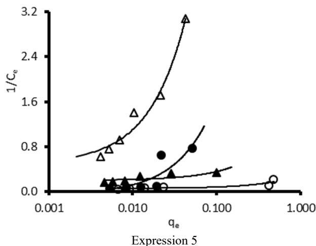
Fig. 3. Adsorption isotherm of chlorantraniliprole and dinotefuran in clay loam and sandy loam soil fitted in different expressions of Langmuir model. Chlorantraniliprole in clay loam soil ● and in sandy loam soil ○; dinotefuran in clay loam soil ▲ and in sandy loam soil Δ.
