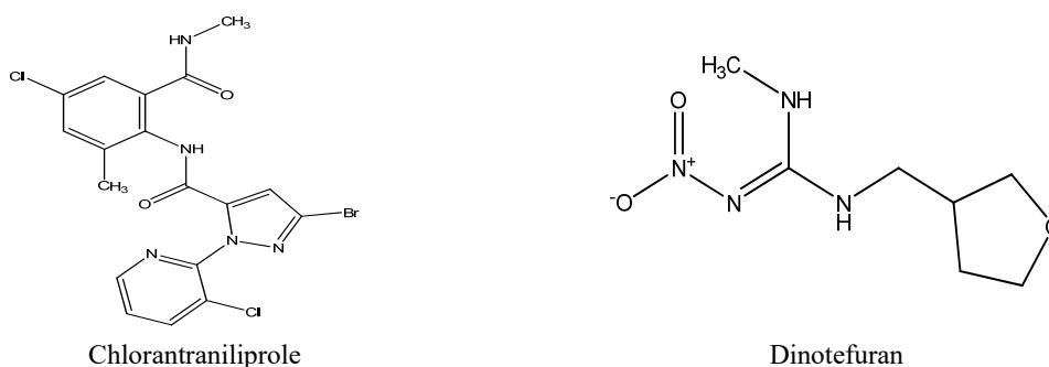
Fig. 1. Chemical structures of tested insecticides.
