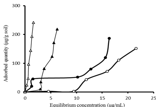
Fig. 2. Adsorption isotherm of chlorantraniliprole and dinotefuran in clay loam and sandy loam soil. Chlorantraniliprole in clay loam soil ● and in sandy loam soil ○; dinotefuran in clay loam soil ▲ and in sandy loam soil △.
