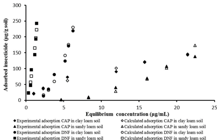
Fig. 5. Comparison of the experimental and calculated adsorption Freundlich data of CAP and DNF on clay loam and sandy loam soil.
