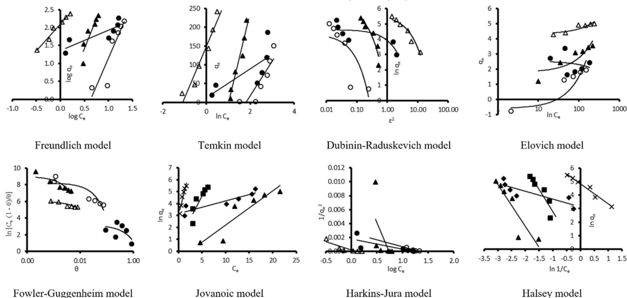
Fig. 4. Adsorption isotherm of tested insecticides in clay loam and sandy loam soil fitted in different adsorption mathematical models. Chlorantraniliprole in clay loam soil ● and in sandy loam soil ○; dinotefuran in clay loam soil ▲ and in sandy loam soil △.
